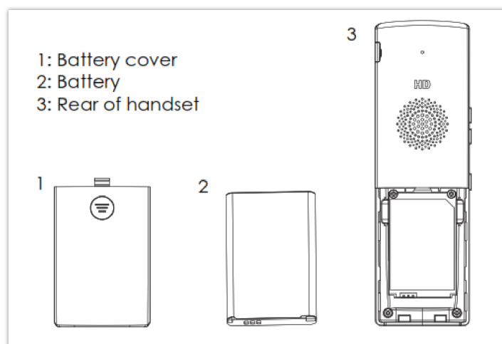
WP820 Handset Setup
