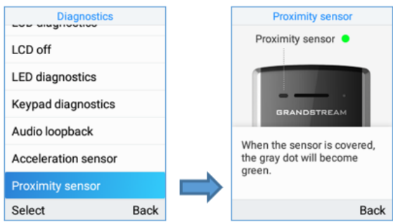
Proximity sensor
